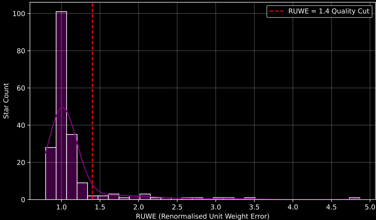
GAPOGEE DR17 Field [191+28_MGA] RUWE Distribution (n= 194)
