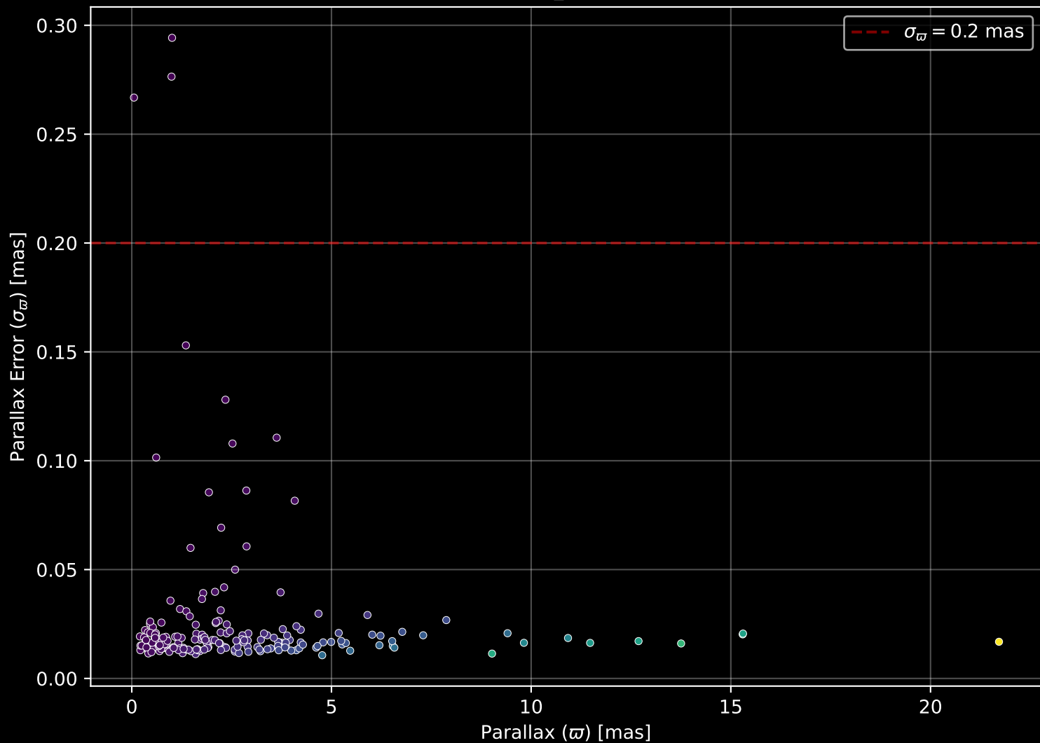
APOGEE DR17 Field: [191+28_MGA] Parallax Quality (n= 204)
