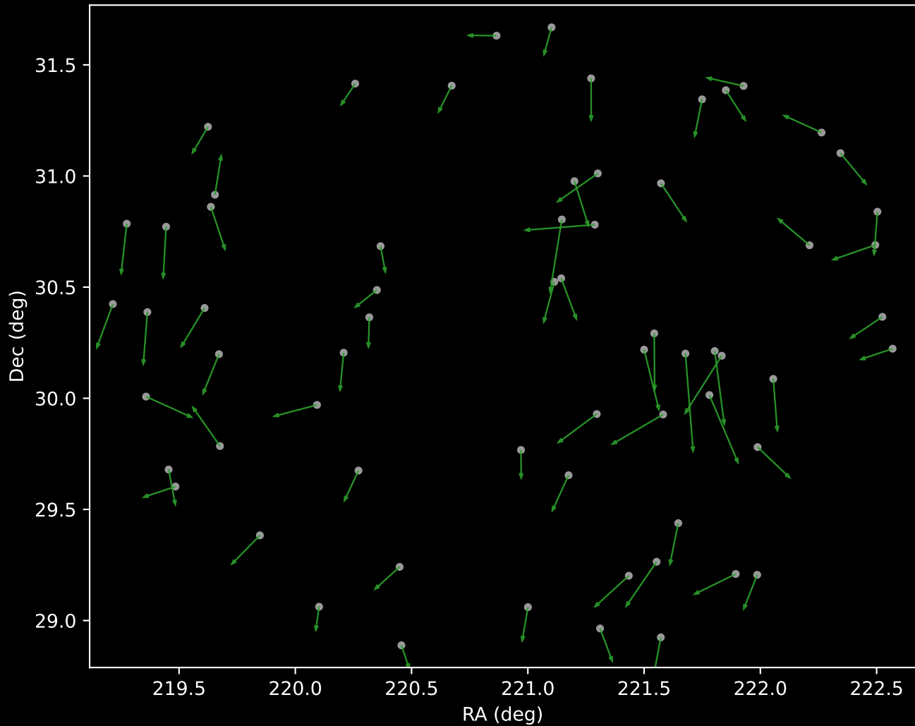
APOGEE DR17 Cluster 4 Proper Motion Vectors (n=65)
