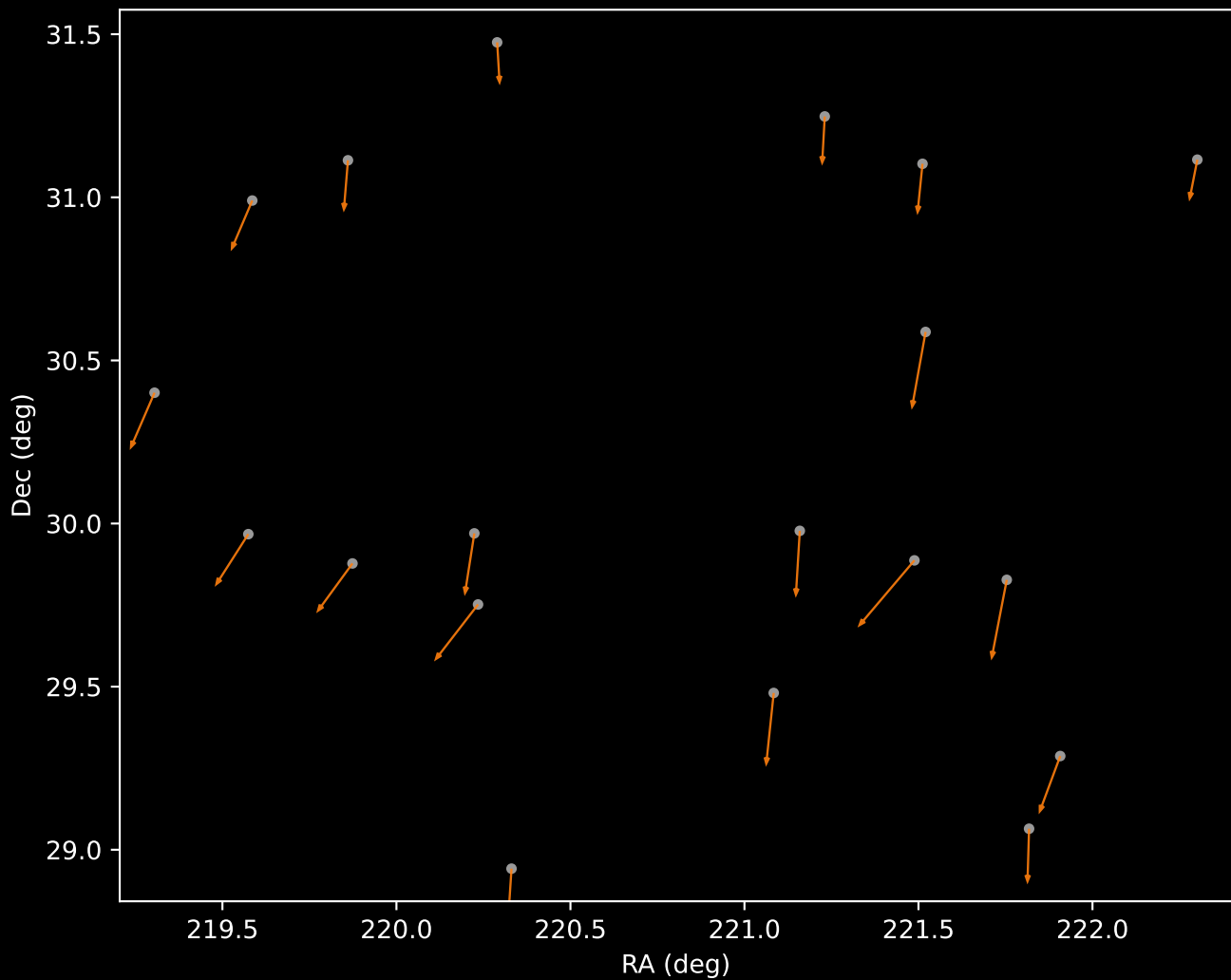
APOGEE DR17 Cluster 2 Proper Motion Vectors (n=19)
