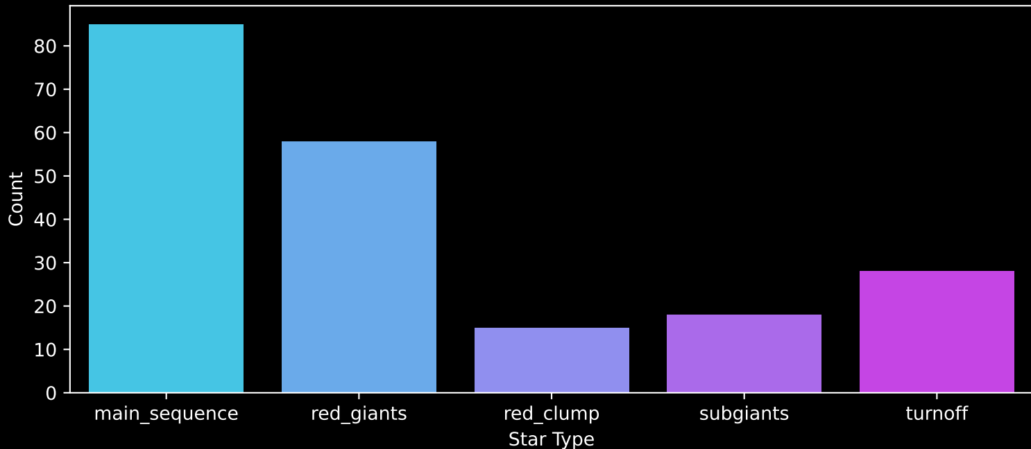
APOGEE DR17 Field: [191+28_MGA] Count plot of Star Type
