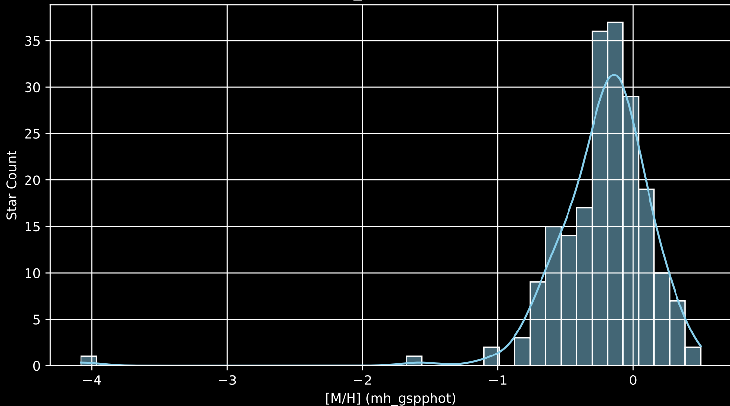
APOGEE DR17 Field: [191+28_MGA [M/H] (mh_gspphot) (n= 202)
