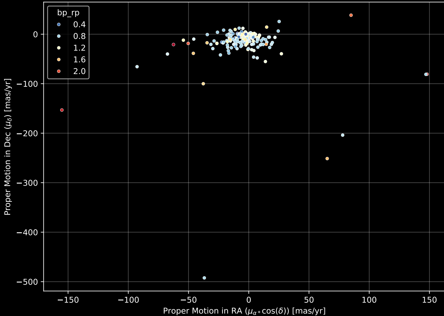
APOGEE DR17 Field: [191+28_MGA] Proper Motion Diagram (n= 204)
